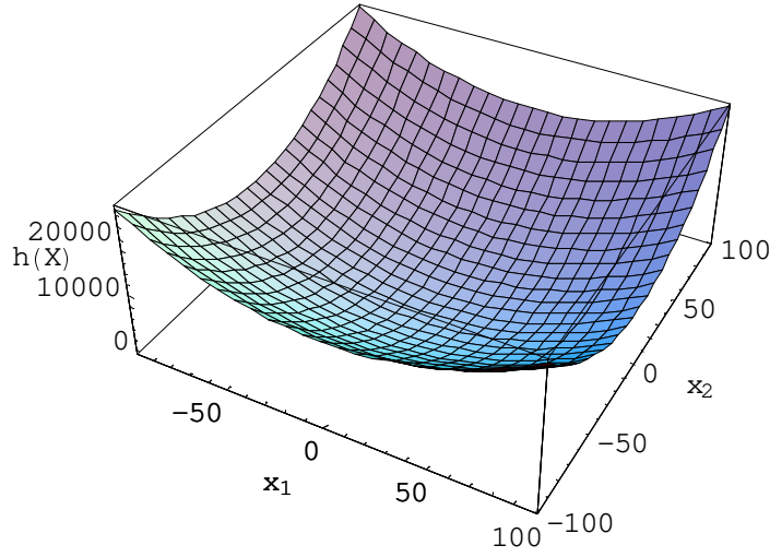
Figure 3.8. A 3-D representation of the log-likelihood ratio function of x_1 and x_2 after simultaneous diagonalization for the two covariance matrices \Sigma_1 and \Sigma_2 .
