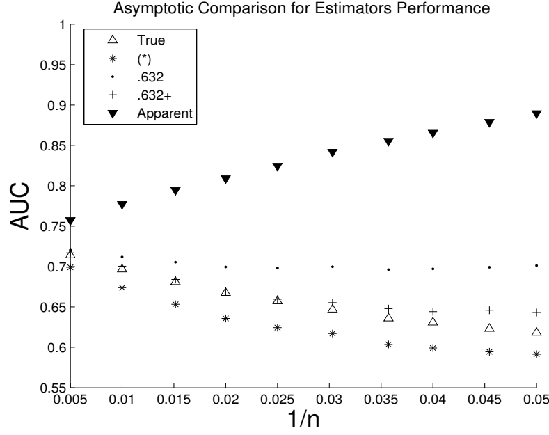
Figure 3.13. Comparison of the three bootstrap estimators, \widehat{AUC}_t^{(*)} , \widehat{AUC}_t^{(.632)} , and \widehat{AUC}_t^{(.632+)} for 5-feature predictor. The \widehat{AUC}_t^{(*)} is downward biased, while the \widehat{AUC}_t^{(.632)} is an over correction for that bias. \widehat{AUC}_t^{(.632+)} is almost the unbiased version of the \widehat{AUC}_t^{(.632)} .
