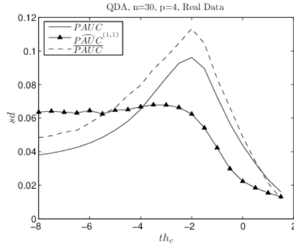
Figure 5.7. Standard error of PAUC , \widehat{PAUC}^{(1,1)} , and \overline{PAUC} vs. th_c using real data set with QDA, n = 30 , and p = 4 .
