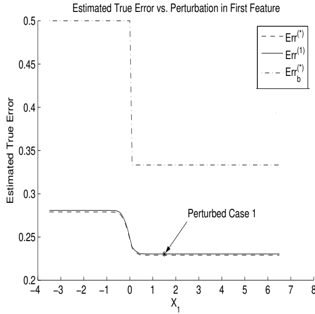
Figure 3.17. The two estimators \widehat{Err}_{\mathbf{t}}^{(*)} , \widehat{Err}_{\mathbf{t}}^{(1)} , and the component Err_{\mathbf{t}^*b}(\widehat{F}_{\varepsilon,i}^{(*)}) estimated after training on the first bootstrap replicate. The first two are smooth while the third is not. The estimated true error is plotted vs. change in the value of the first feature.
