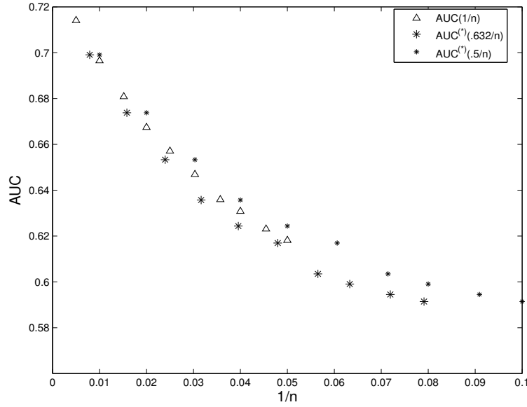
Figure 3.14. The true AUC and rescaled version of the bootstrap estimator \widehat{AUC}_{\mathbf{t}}^{(*)} . At every sample size n the true AUC is shown along with the value of the estimator \widehat{AUC}_{\mathbf{t}}^{(*)} at n/.632 and n/.5 .
